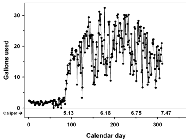
Figure 9. Daily ET A of red maple in a #300 container.
