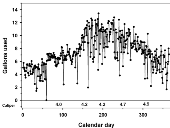
Figure 3. Daily ET A of 'Nellie R. Stephens' holly in a #300 container.
