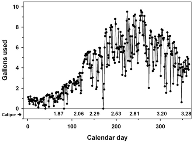
Figure 5. Daily ET_A of Live oak in a #95 container.
