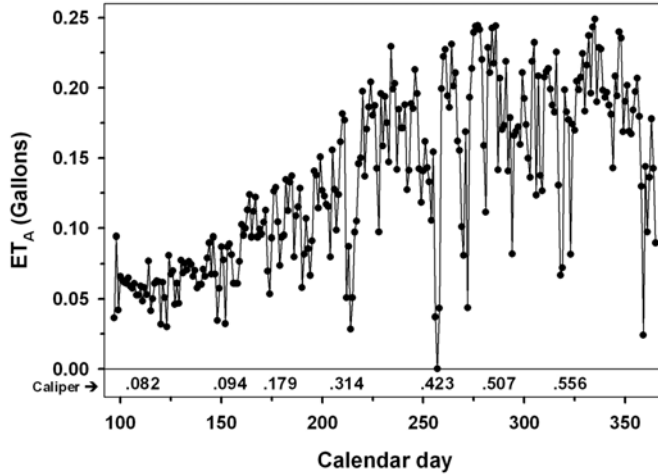
Figure 4. Daily ET_A of Live oak in a #7 container.
